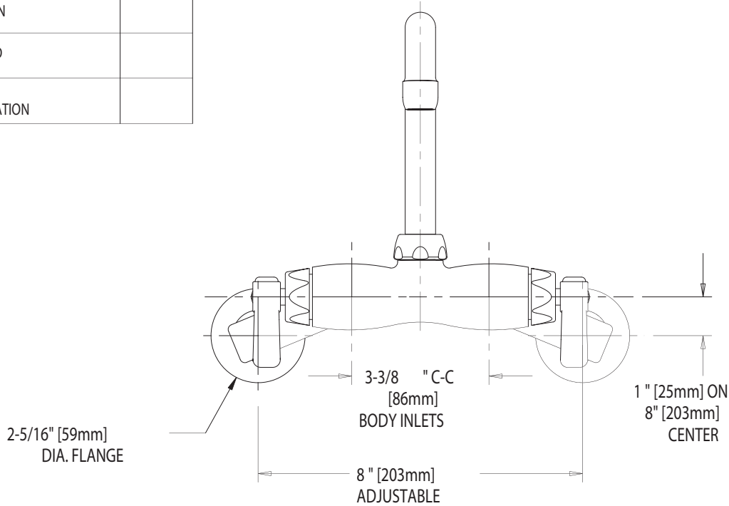
FRONT VIEW
