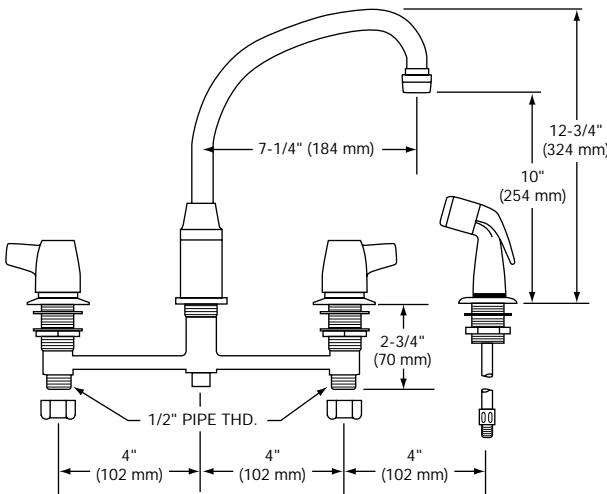
LKC2433 Illustrated
