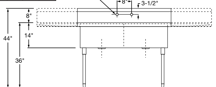
1-1/2" DIA. 2 HOLES
