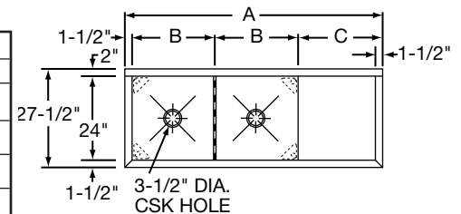
RIGHT DRAINBOARD
